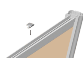
T形件安装 Plastic accessory installation
