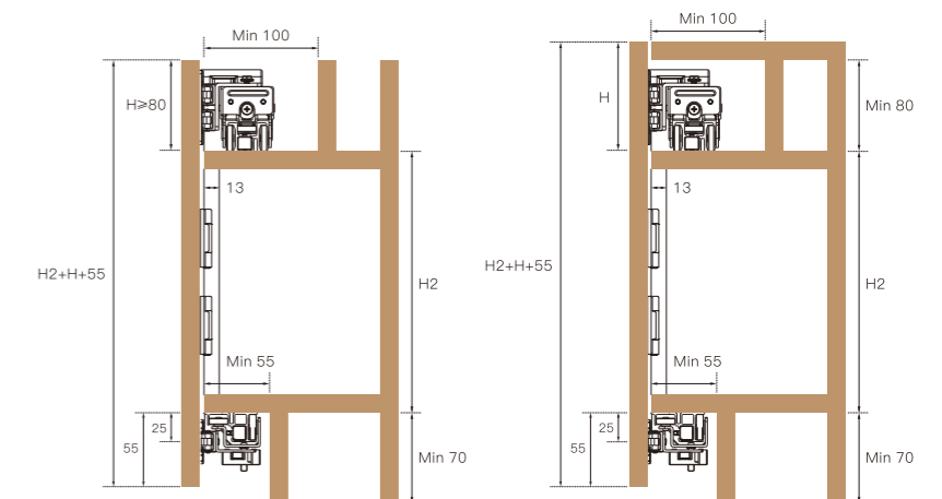
不装顶柜 Without top cabinet
