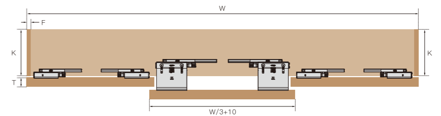
三门双缓冲(三门带对碰) Full soft close for 3 doors
