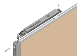
缓冲器安装 Damper installation
