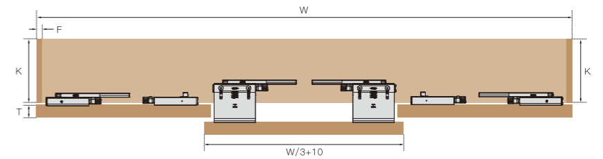
三门双缓冲 Double soft close for 3 doors
