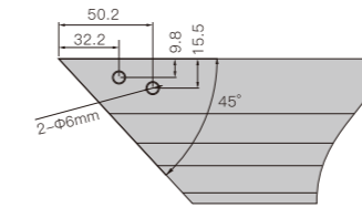
铝框开孔尺寸 Hole size on frame
