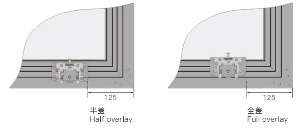
定位滑轮区分门板半盖轨道与全盖轨道 Half overlay and Full overlay
