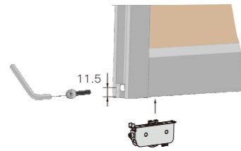
滑轮安装 Runner installation
