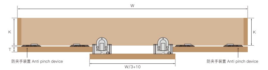
前门在中间 Outer door is in the middle
