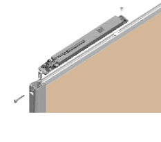
缓冲器安装 Damper installation
