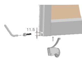
滑轮安装 Runner installation
