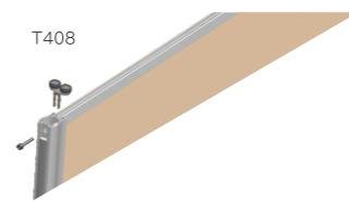
上滑轮安装 Upper runner installation
