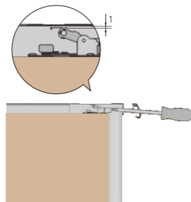
408B上滑轮调节 Anti-jumping upper runner adjustment
