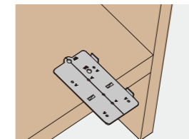
预钻下轨安装孔 Drill holes for down rail
