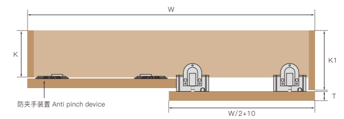
前门在右 Outer door is on the right
