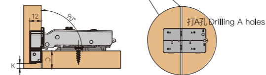
H94直臂铰链盖位对照表 Coverage calculation table
