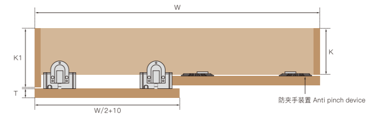
前门在左 Outer door is on the left
